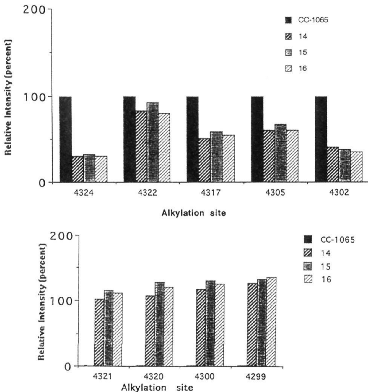
Figure 5. (Upper panel) A comparison in the form of a histogram of the relative extents of alkylation at A residues at major recognition sites by CC-1065 and the synthetic analogues 14, 15, and 16 in the region 4302–4324. (Lower panel) A comparison in the form of a histogram of the relative extents of alkylation at G residues at minor recognition sites by CC-1065 and 14, 15, and 16 in the region 4299–4321.
