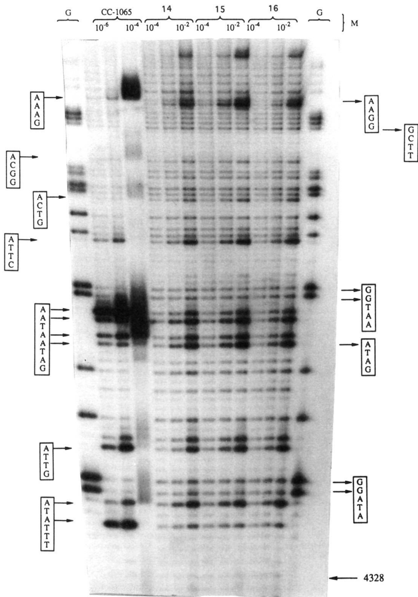
Figure 4. Autoradiogram of thermally induced cleavage pattern induced on a portion of the 5'-labeled pBR322 restriction fragment by CC-1065 and the synthetic CI analogues 14, 15, and 16 at the concentrations indicated. G represents the Maxam-Gilbert G cleavage.
