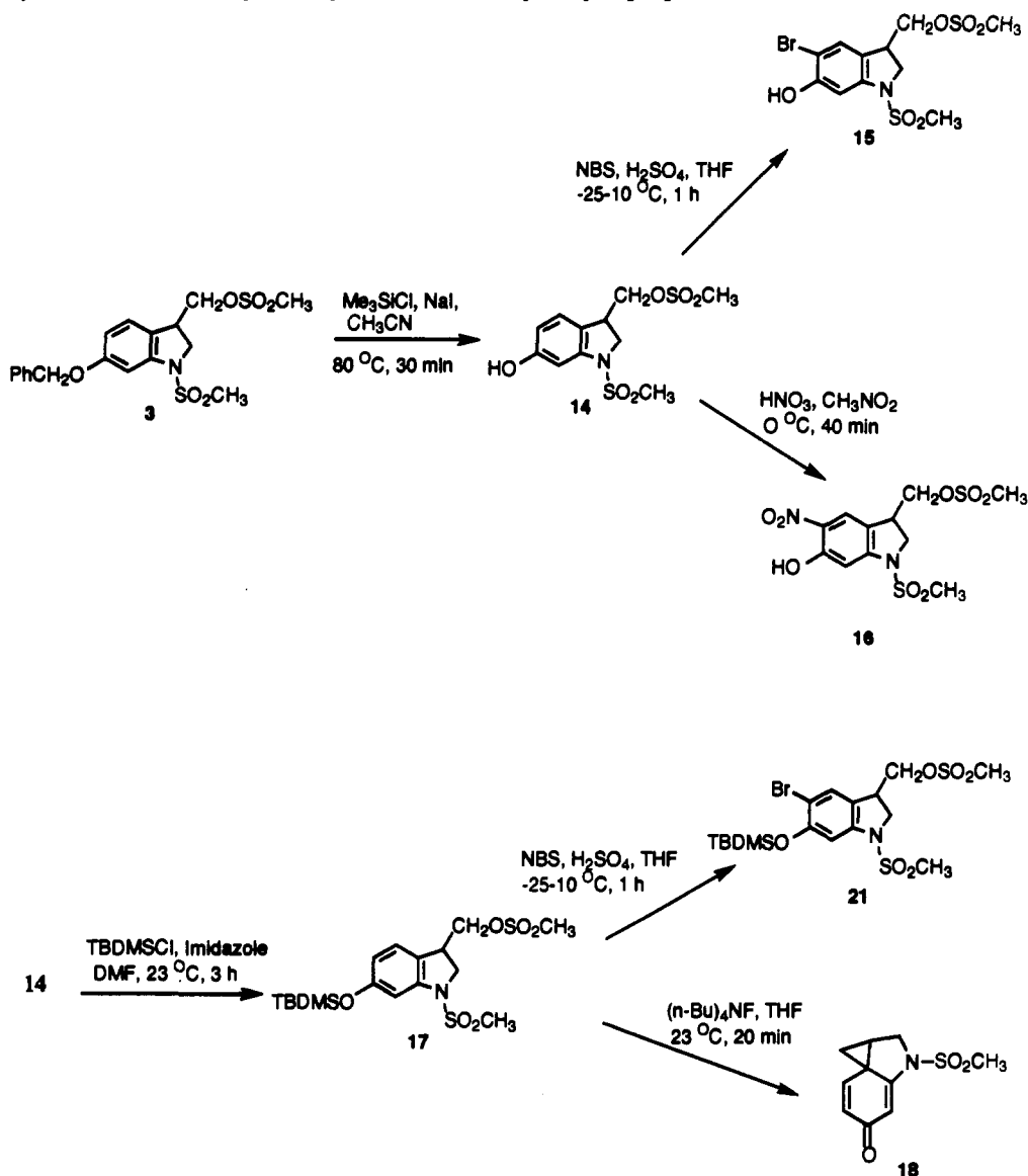
Scheme III. Synthesis of N -(Methylsulfonyl)-1,2,7,7a-tetrahydrocycloprop[c]indol-4-one (18)
