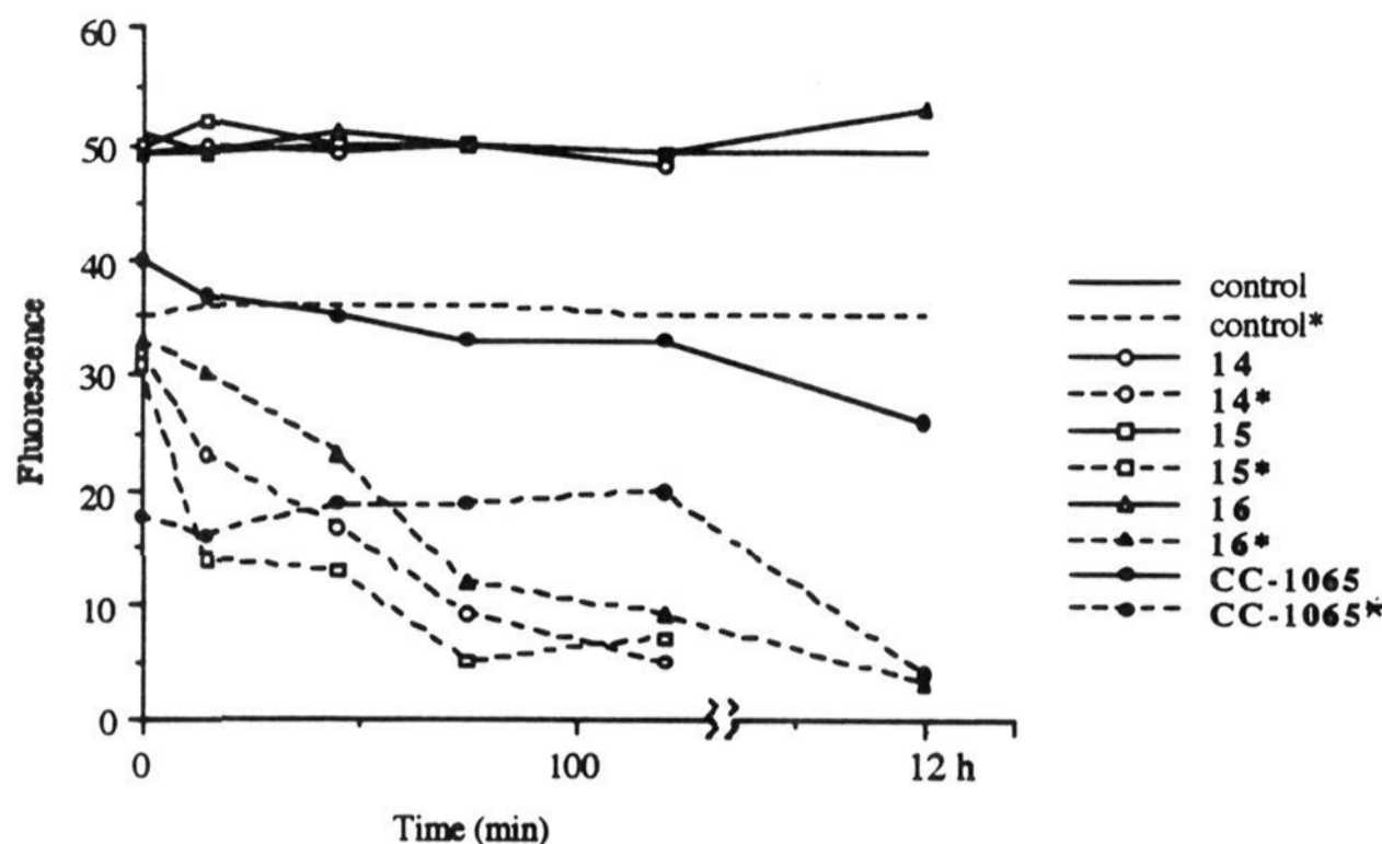
Figure 2. Time dependence of the effects of individual drugs on conversion of PM2 CC-DNA to OC form reflected in the change in fluorescence of bound ethidium. A 100- \mu L sample of DNA at 1 A_{260} was reacted with the drugs at 80 \mu M in buffer of pH 8.0. 10 \mu L of samples were then pipetted into 2 mL of the pH 12 assay solution in the indicated intervals. The fluorescence was first read at room temperature and the solution then heated at 95 ^{\circ} C for 5 min before the second reading (* marked).
