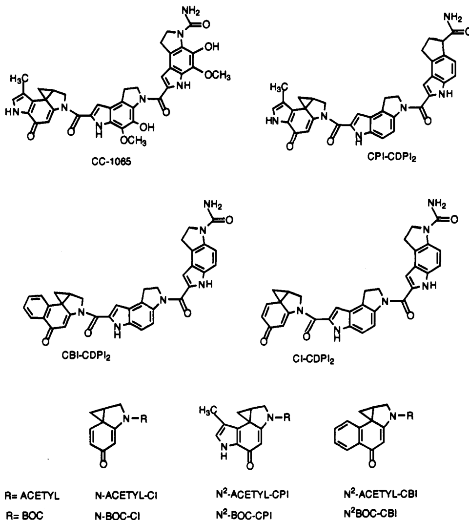
Figure 1. Structures of the antitumor antibiotic CC-1065 and synthetic analogues.
