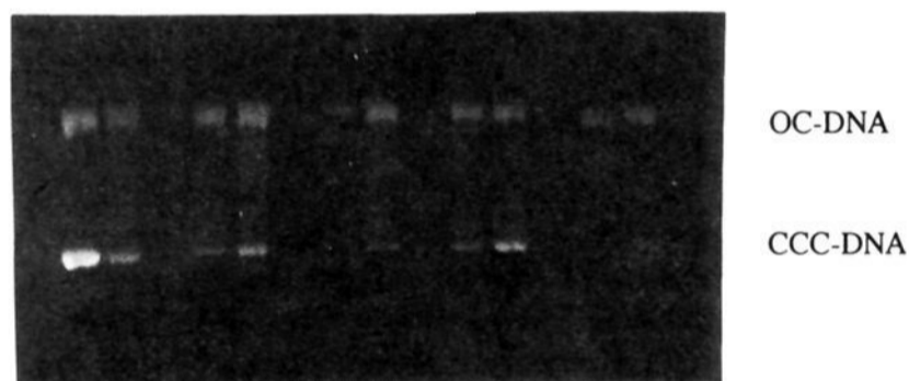
Figure 3. Agarose gel electrophoresis of the reaction mixture of PM2 DNA 0.7 A_{260} with drugs in varying concentrations. The drugs were incubated with DNA for 20 h at room temperature, and the solutions were then heated at 95 ^{\circ} C for 5 min before loading on gels. (a) control (without drug, before heating); (b) control (without drug, after heating); (c-e) 80 \mu M, 8 \mu M, 0.8 \mu M of 14; (f-h) 80 \mu M, 8 \mu M, 0.8 \mu M of 15; (i-k) 80 \mu M, 8 \mu M, 0.8 \mu M of 16; (l-n) 80 \mu M, 8 \mu M, 0.8 \mu M of CC-1065.
